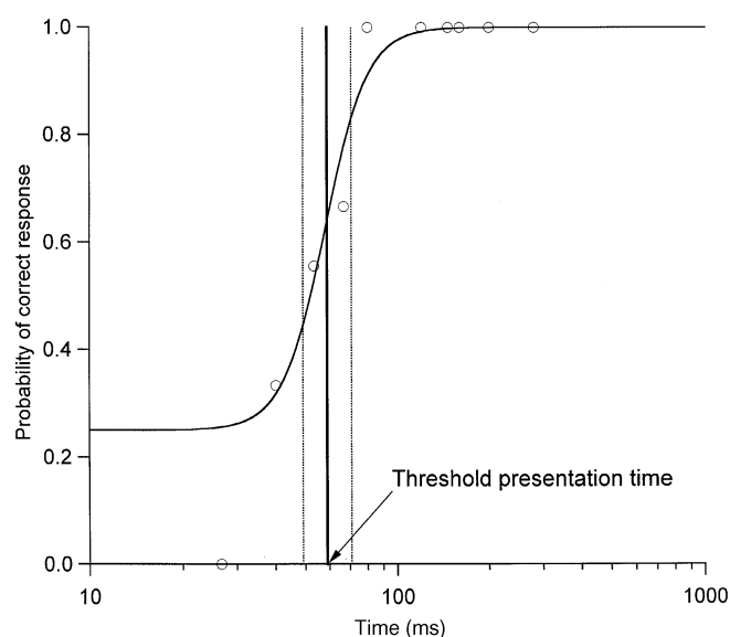
Fig. 3 Example of the psychometric function fit to the probability of a correct response as a function of the stimulus duration (on log scale). The S-shaped function is the cumulative normal logistic function and the solid vertical line intersects this function at its steepest point. This point corresponds to the Best-PEST estimate of the threshold. The dotted lines show \pm 1 SE of this estimate.
